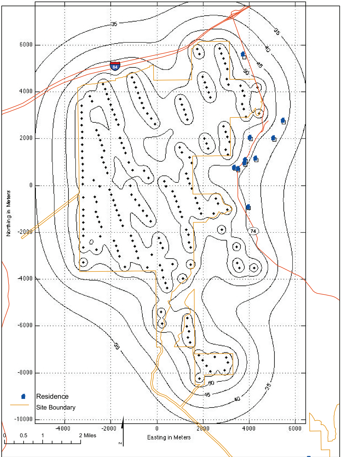
Figure RAI#2 X1a Noise Contours - 192 Wind Turbines at 109.2 dB LWA
